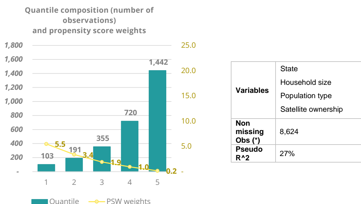
Figure 114: PSW model: explanatory variables, statistics, quantile composition, and weights
